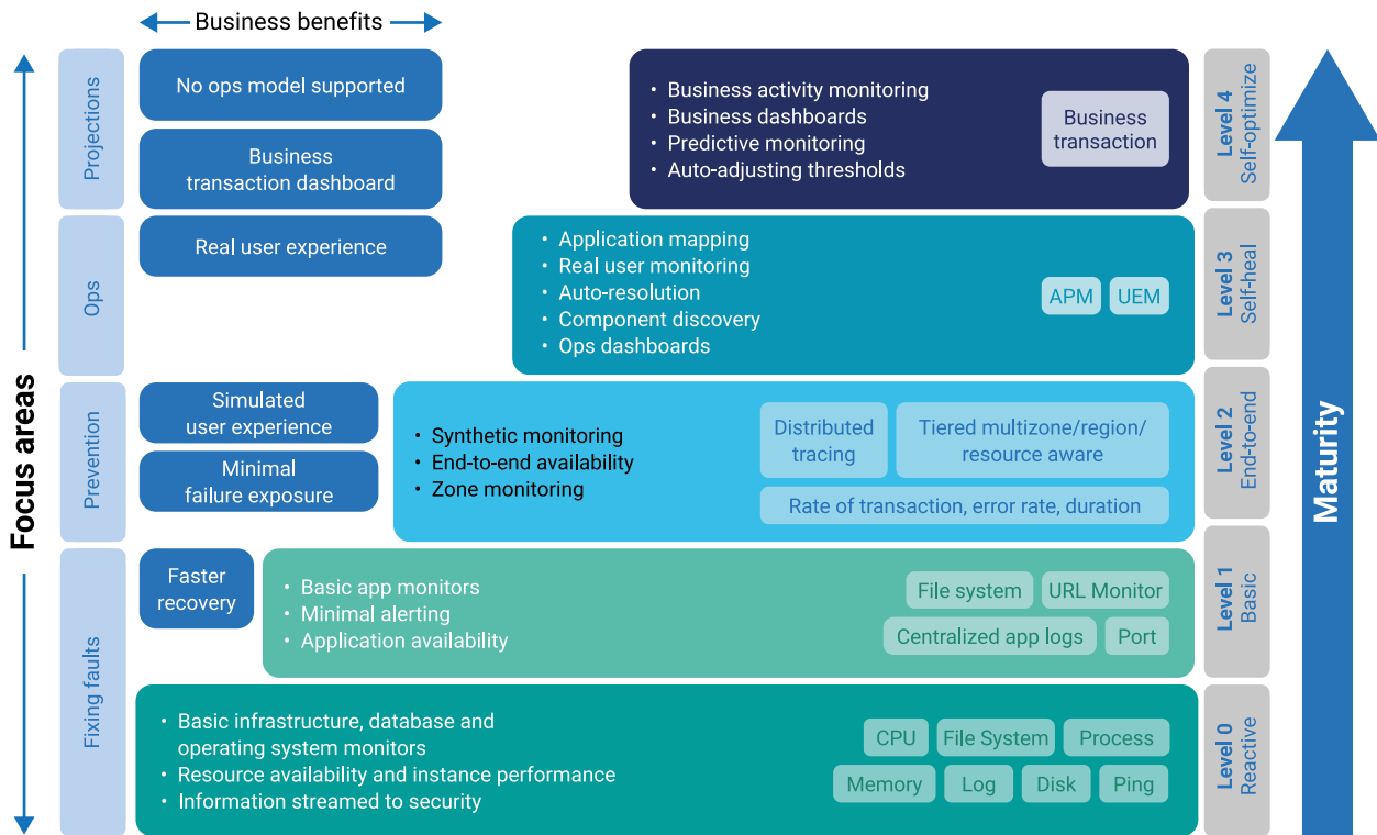
Figure 1: Performance observability maturity model
